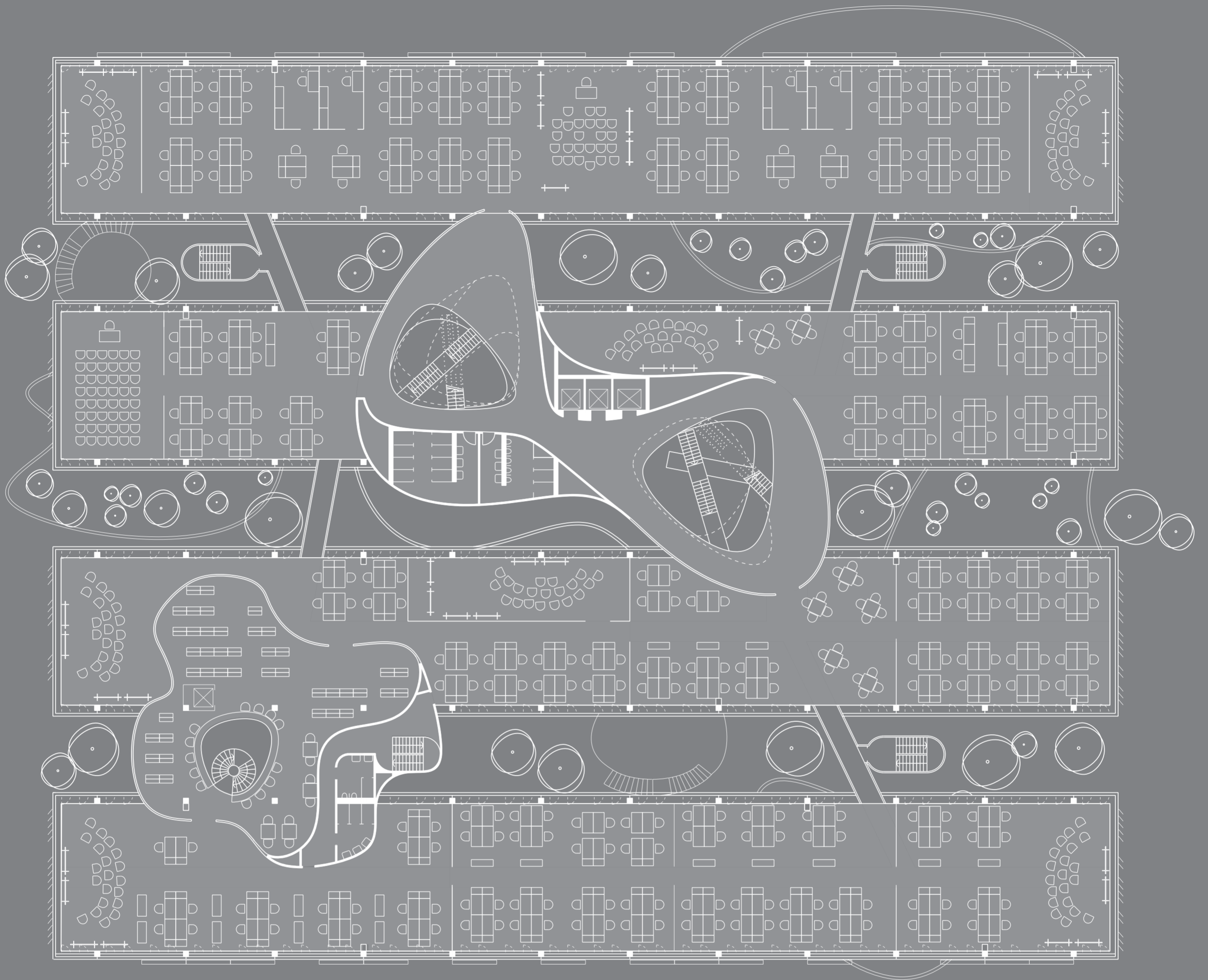
first floor 1/250
